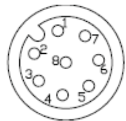
Bottom view (male connector)
