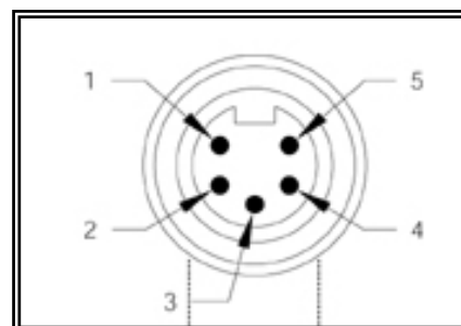
Bottom view (male connector)
